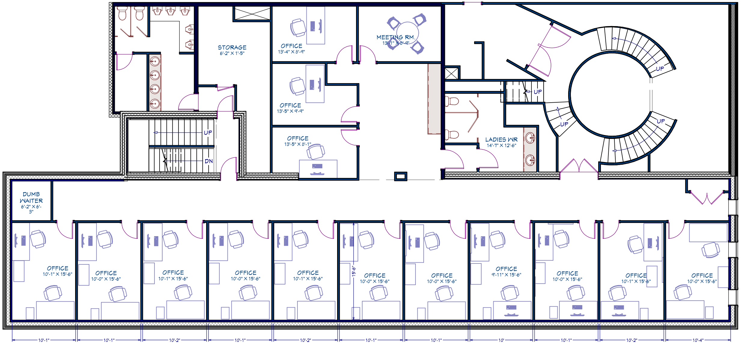
OFFICE PLAN
